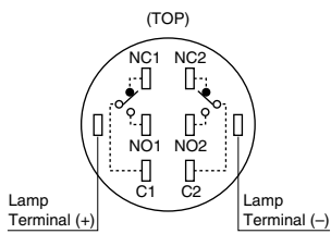
Illuminated Pushbutton
