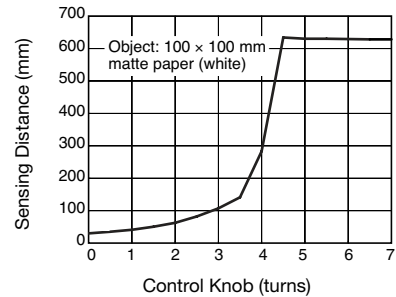
Control Knob vs. Sensing Distance
